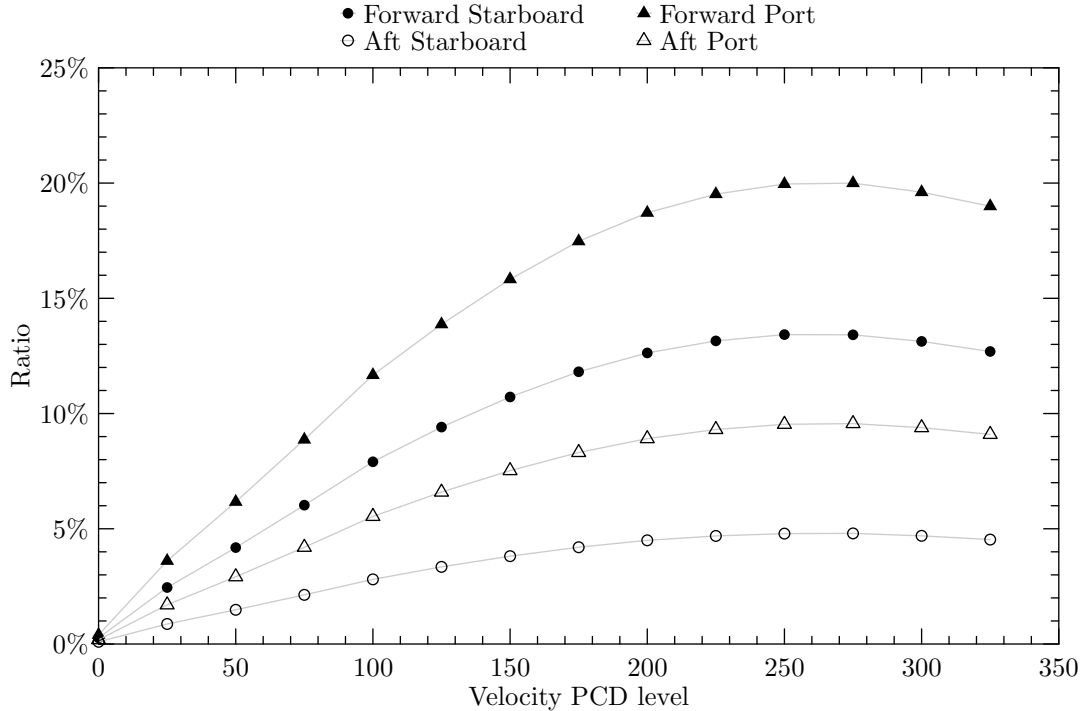
Figure 7: Velocity Pockels-cell driver scan made at 2009 July 11 06:30 UTC.
