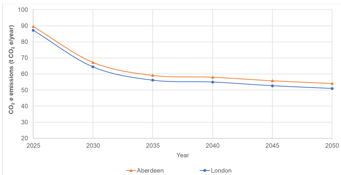
Figure 21. Impact of grid carbon emission factor change on total carbon emitted by the 600 m 2 supermarket in the 2 locations studied.
