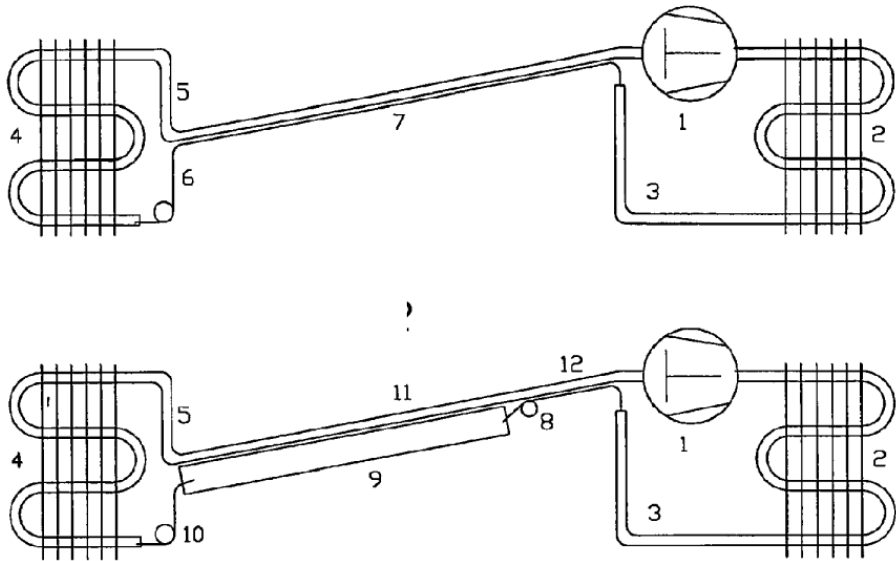
Figure 37. TFC concept (upper diagram conventional capillary system, lower diagram TFC system) Zimmermann, 2008
