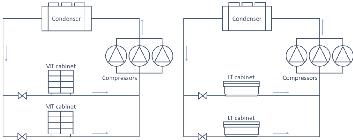
Figure 6. Simple direct expansion (DX) system.
