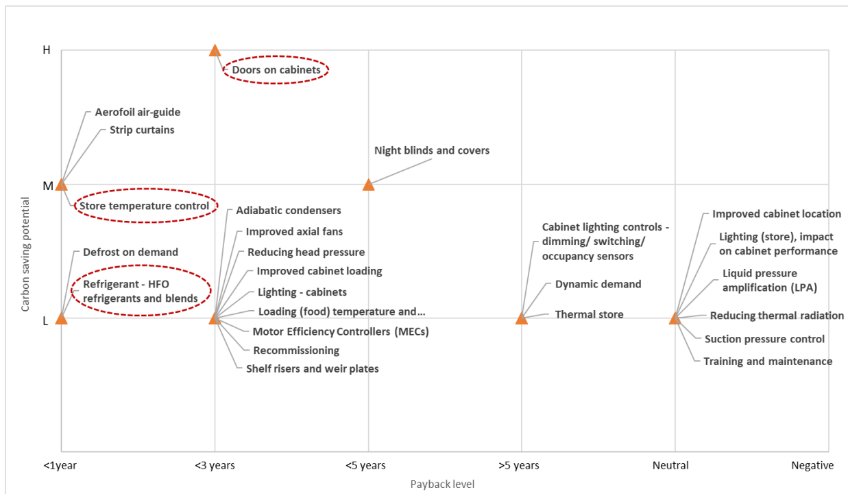
Figure 11. Refrigeration minor retrofit options.
