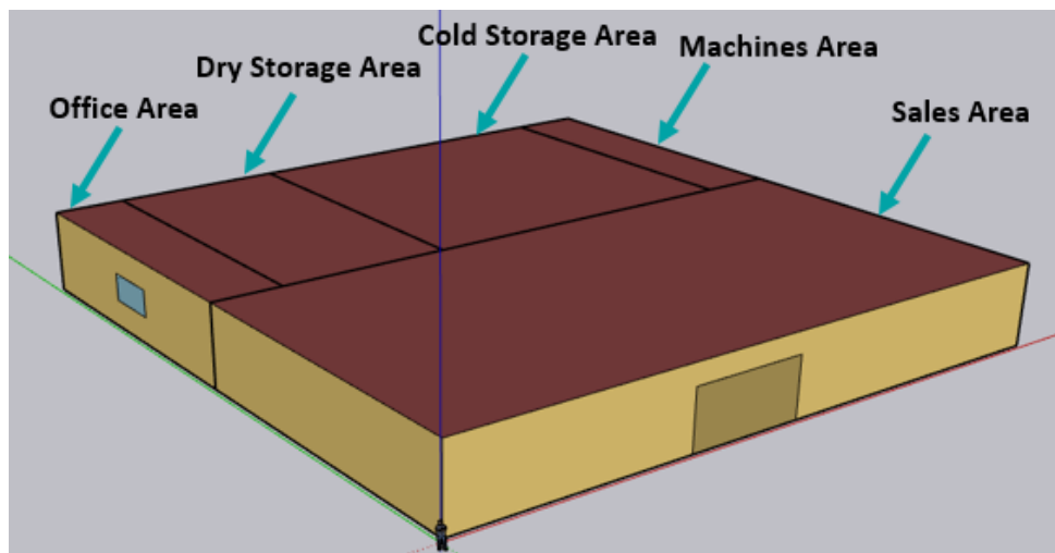
Figure 54. Geometry of the MS supermarket with its space types
