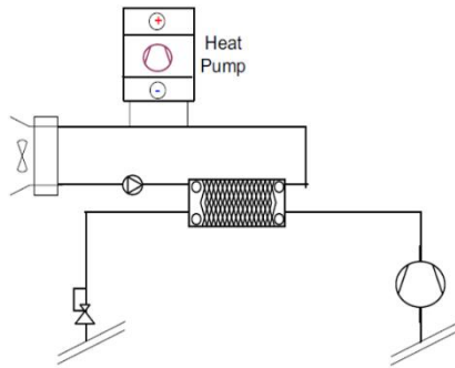
Figure 48: Simplified scheme of a heat recovery with a cascade system 606
