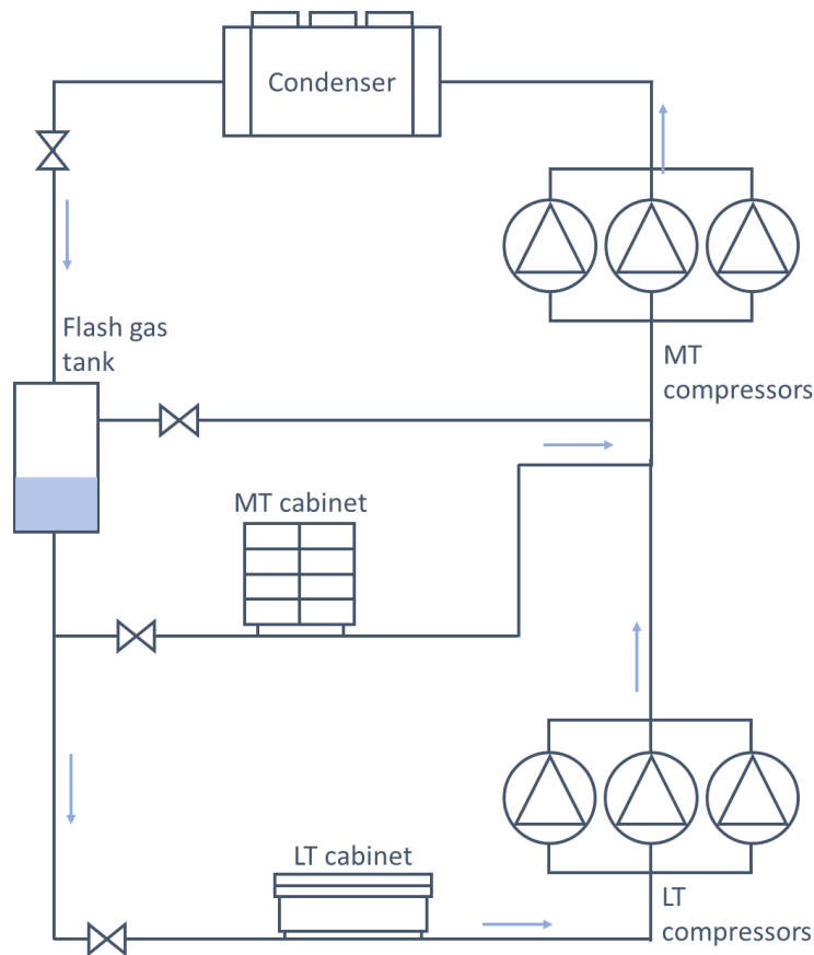
Figure 57. Adding a refrigeration system for the supermarket
