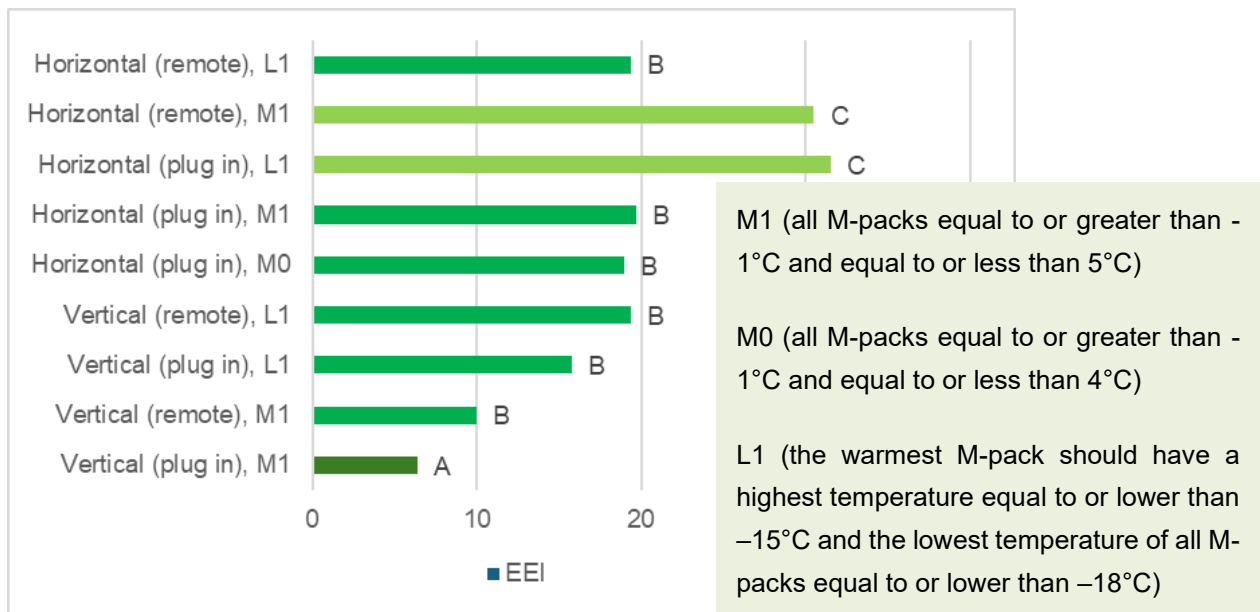
Figure 9. Most efficient refrigerated cabinets listed on Topten.
