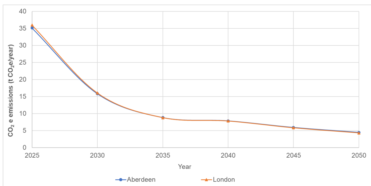
Figure 26. Impact on carbon emissions of the combined minor retrofit options for the 2,100 m 2 stores in the 2 locations from 2025 to 2050.
