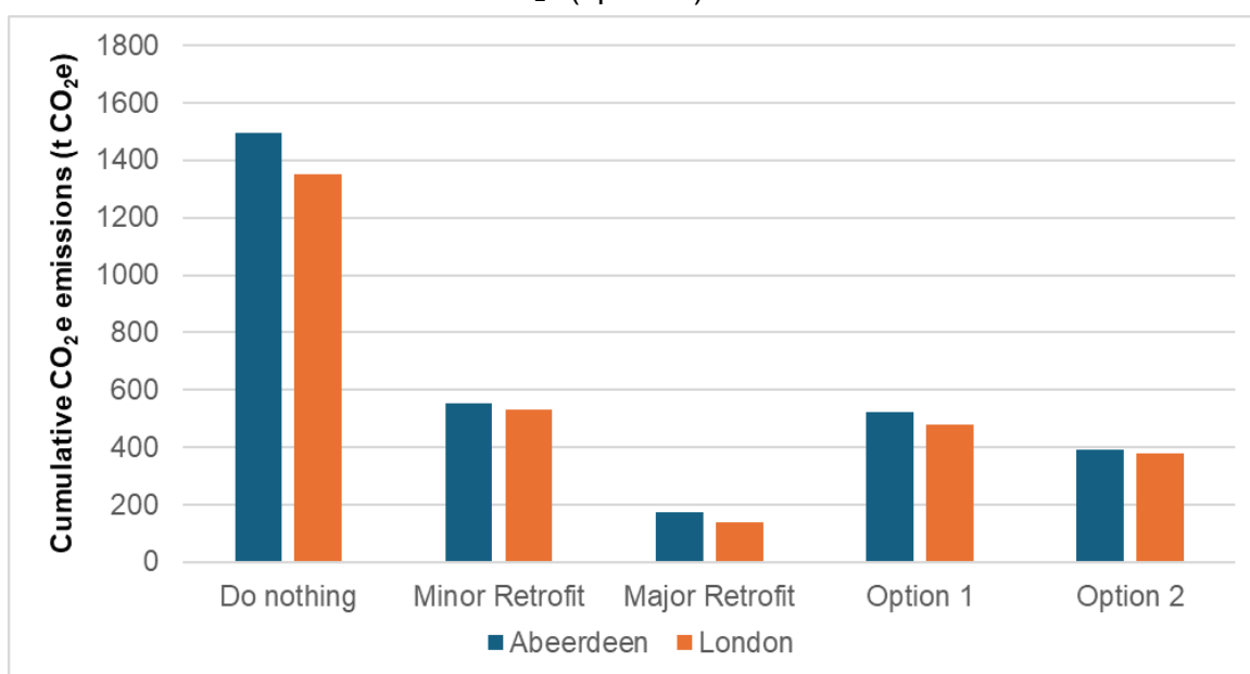
Figure 34. Carbon emitted by the 2,100 m 2 store in different cities from 2025 to 2050.
