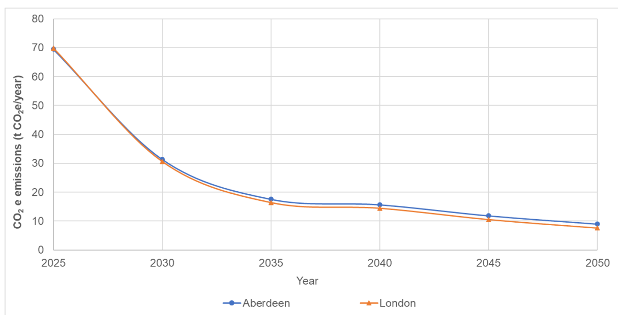
Figure 26. Impact on carbon emissions of the combined minor retrofit options for the 2,100 m 2 stores in the 2 locations from 2025 to 2050.
