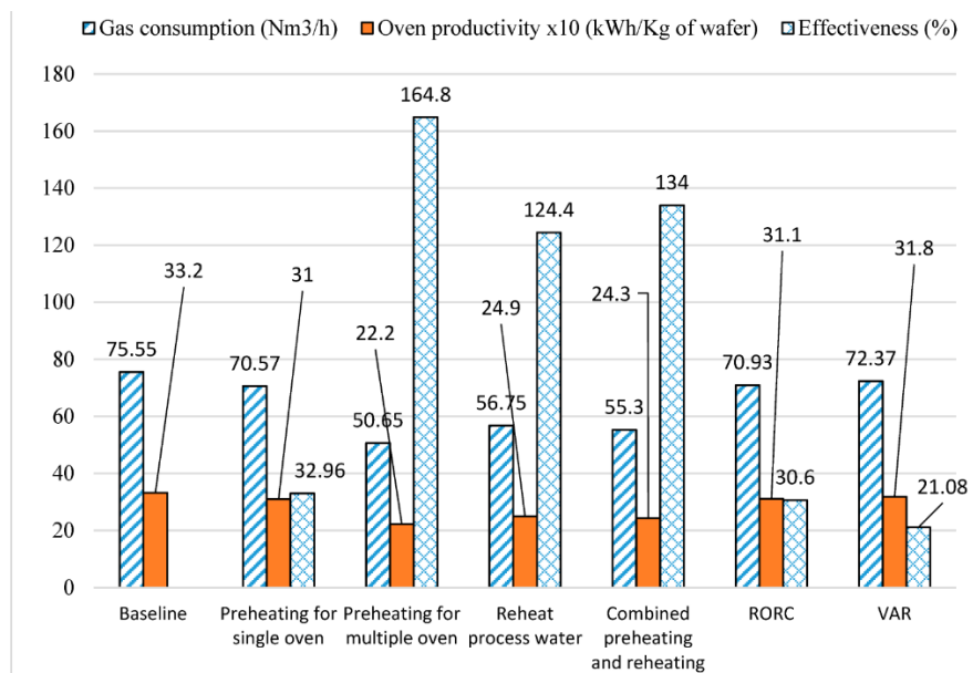
Figure 39. Comparison of heat recovery technologies based on oven's gas consumption, productivity and effectiveness. (taken from Mukherjee et al., 2020).
