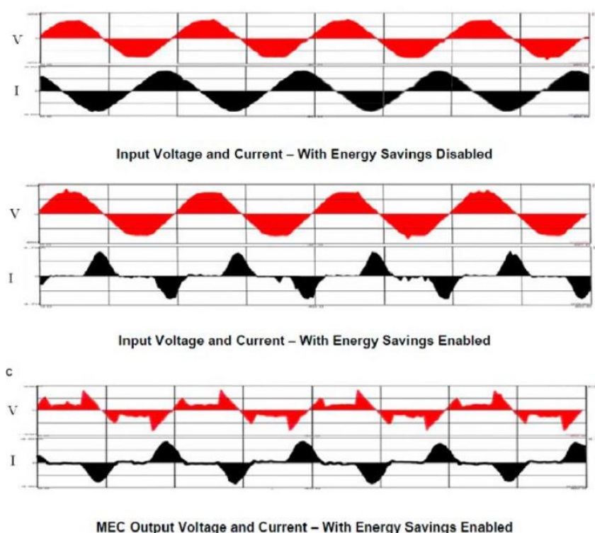
Figure 36. Current & voltage waveforms on single-phase motor both with and without energy savings (Envirostart).
