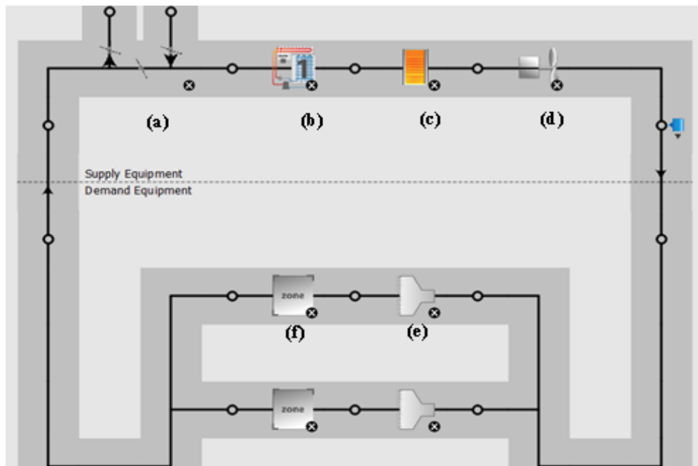
Figure 56. Adding a typical HVAC system for the MS supermarket: (a) Outside air system, (b) Cooling coil, (c) Electric heating coil, (d) Fan, (e) Zone terminal units, (f) Zone
