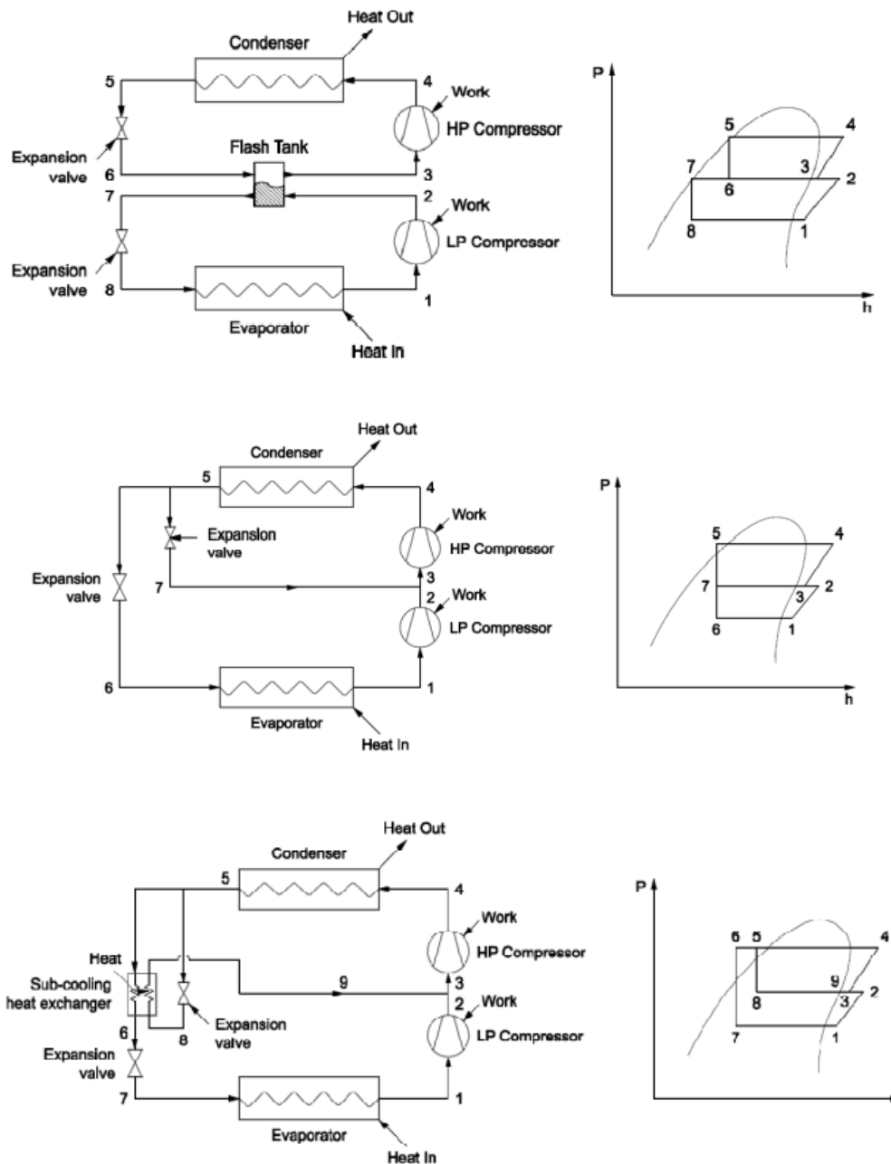
Figure 38. Three two-stage system configurations [Torrella et al (2009)].
