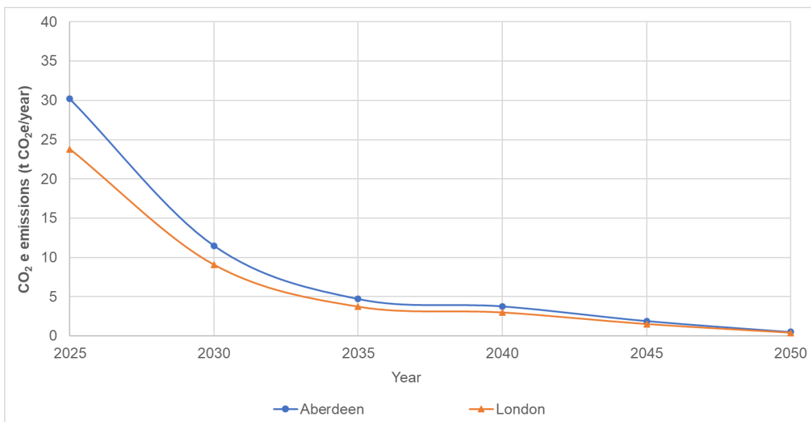
Figure 32. Impact on carbon emissions of the combined major retrofit options for the 2,100 m 2 stores in the 2 locations from 2025 to 2050.
