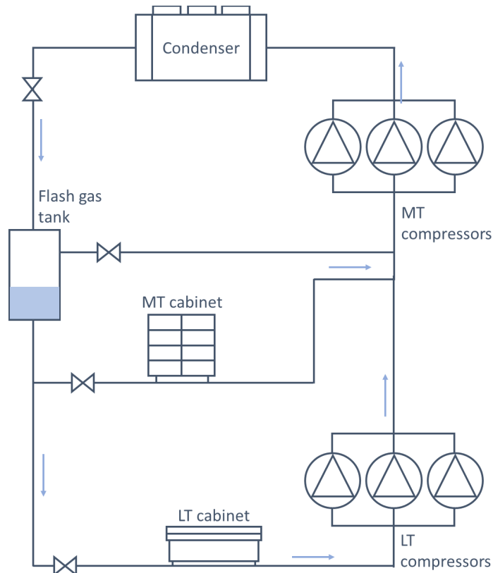
Figure 7. R744 booster system.
