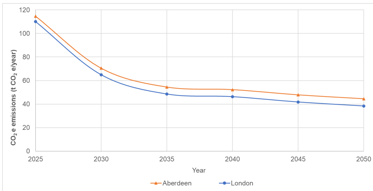
Figure 20. Impact of grid carbon emission factor change on total carbon emitted by the 2,100 m 2 supermarket in the 2 locations studied.
