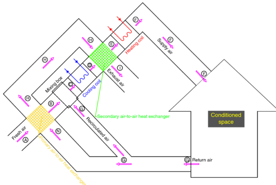
Figure 44: Simplified schema of an air handling unit (AHU) and a conditioned space (e.g. building) 600
