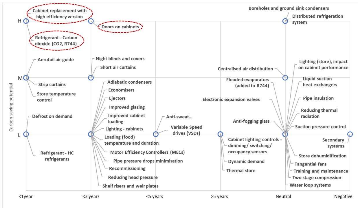
Figure 12. Refrigeration major retrofit options.
