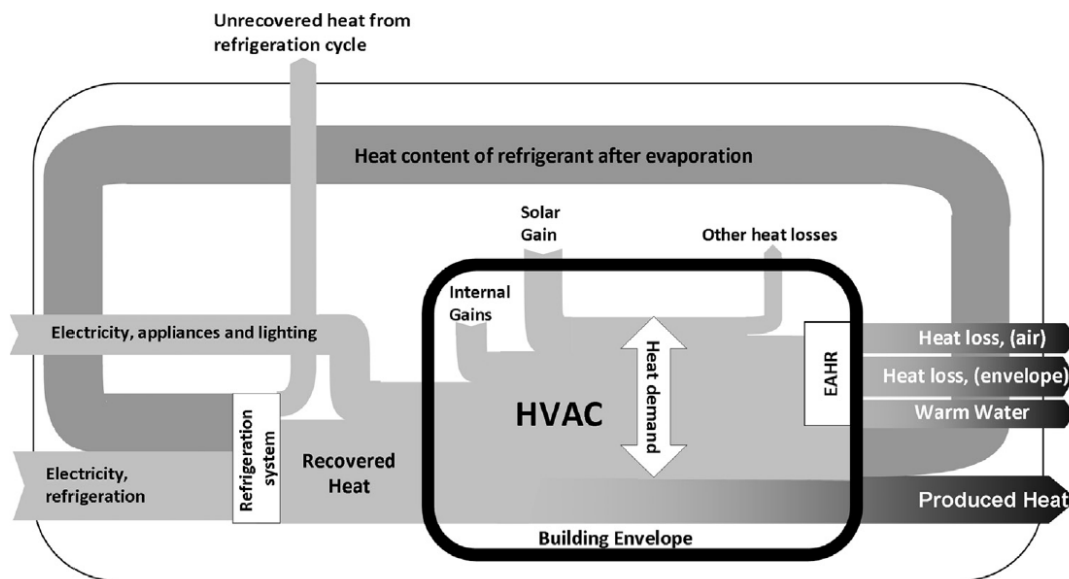
Figure 43: Energy flow diagram of a supermarket including heat recovery (Galvez-Martos et al., 2013)
