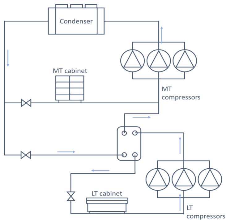
Figure 8. Cascade system.
