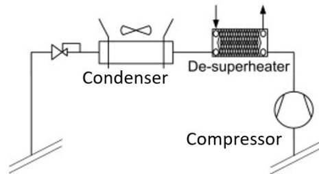
Figure 46: Simple scheme of a direct heat recovery solution via a desuperheater 595
