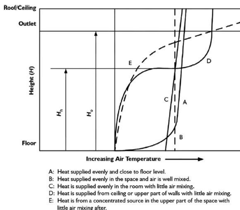
Figure 42. Qualitative characteristic curves of thermal stratification, retrieved from Wang et al. (2019)
