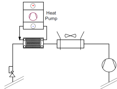
Figure 49: Simplified scheme of a heat recovery by means of a heat pump integrated after the aircooler 598
