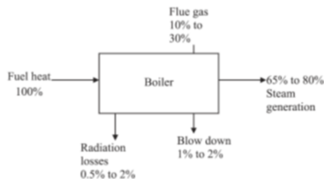
Figure 41. Typical heat balance of a boiler 560
