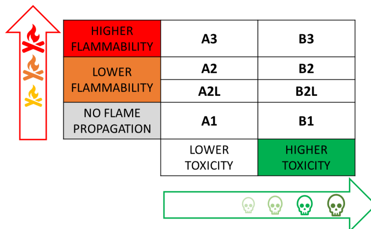
Figure 3. Toxicity and flammability classification of refrigerants.
