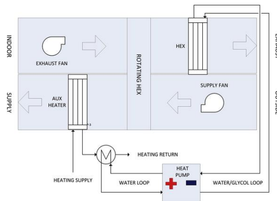
Figure 47: Simplified schema of an AHU with an energy wheel and an additional heat recovery with a heat pump 605
