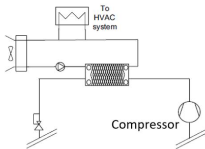
Figure 45: Simple scheme of a direct heat recovery solution via an intermediate circuit and a floating condensation pressure 595
