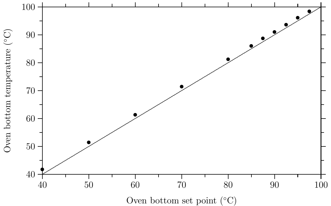
Figure 3: Here is how the measured oven bottom temperature compares to the temperature-controller set points. This run was done on 2005 June 15.
